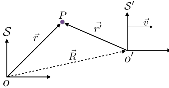
FIGURE 1. Two inertial systems \mathcal{S} and \mathcal{S}' moving relative to each other with velocity \vec{v} . Position vector of a point P in \mathcal{S} is \vec{r} \equiv (x, y, z, t) \equiv x_\mu and that in \mathcal{S}' is \vec{r}' \equiv (x', y', z', t') \equiv x'_\nu .
